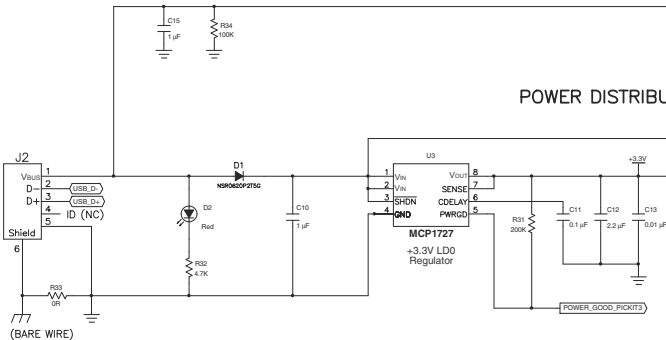
USB INTERFACE (BUS POWERED)
