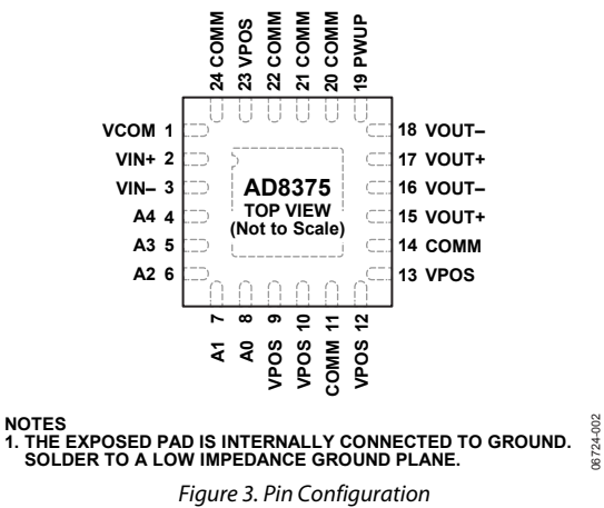
Figure 3. Pin Configuration
