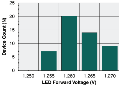
LED Forward Voltage Distribution (N=50, I_F=5mA )
