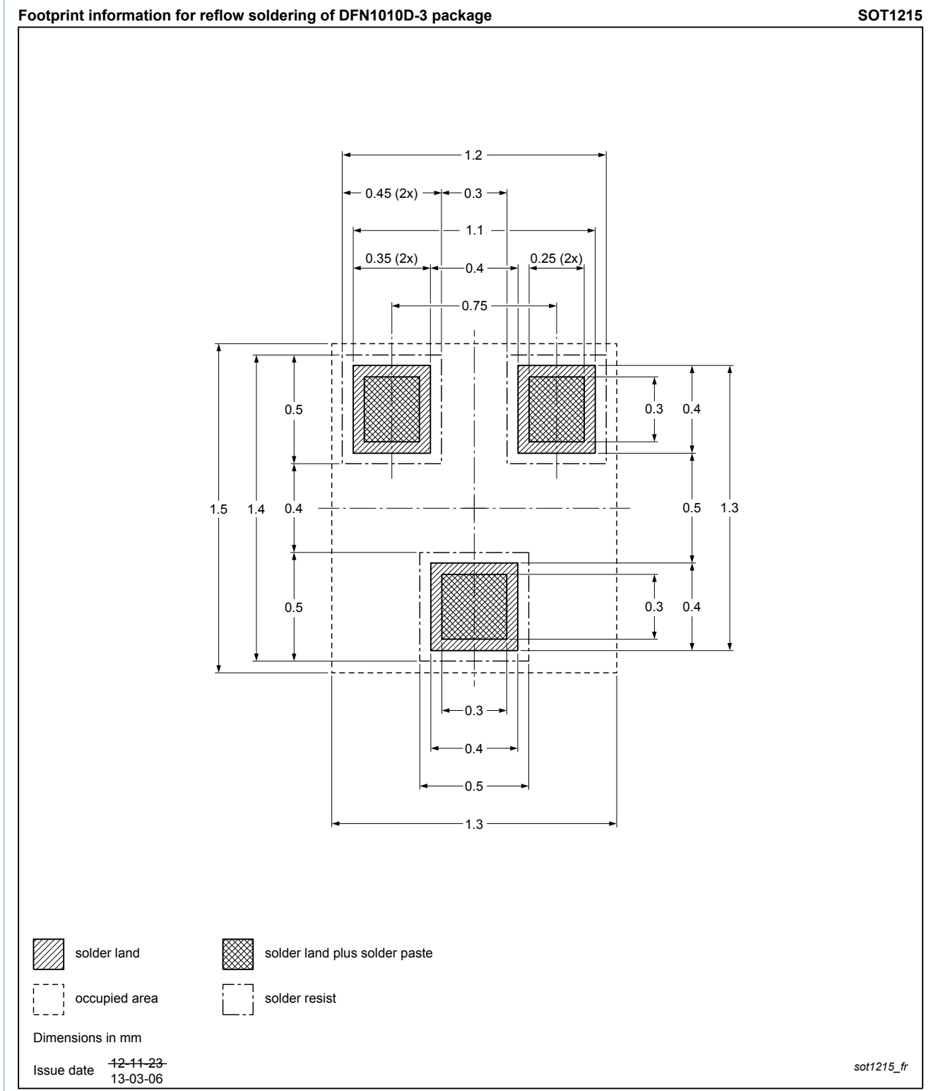
Fig. 12. Reflow soldering footprint for DFN1010D-3 (SOT1215)
