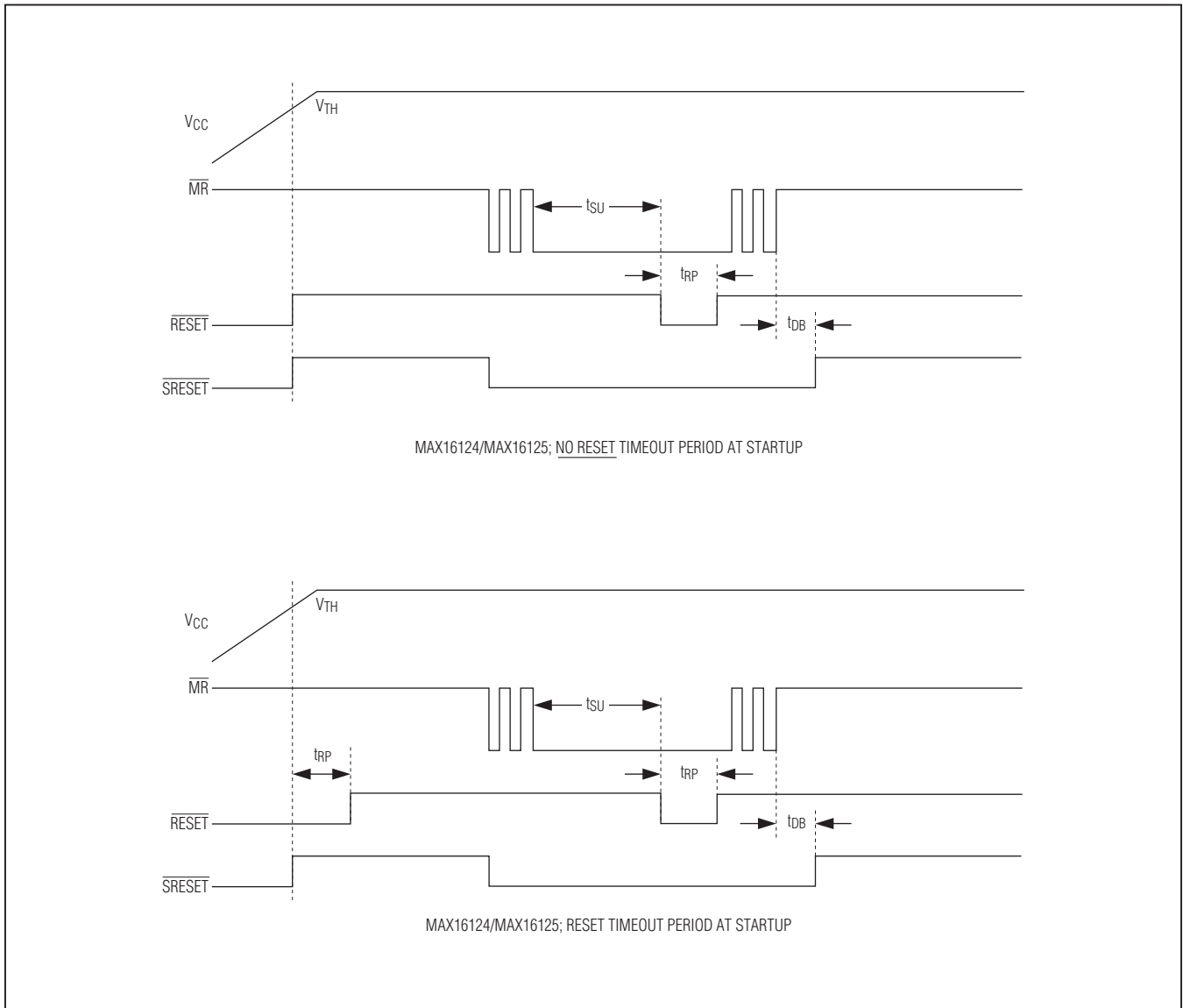
Figure 1b. Timeout Periods at Startup
