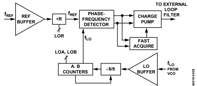
Figure 39. LO Synthesizer
