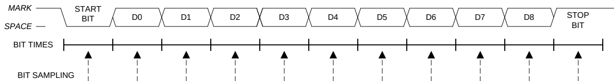
Figure 16.6. UART Modes 2 and 3 Timing Diagram
