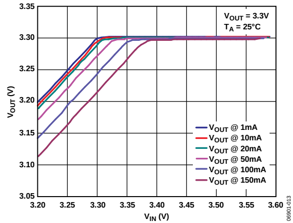
Figure 15. Output Voltage vs. Input Voltage (In Dropout), WLCSP
