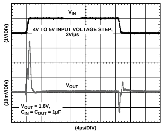
Figure 25. Line Transient Response, Load Current = 150 mA
