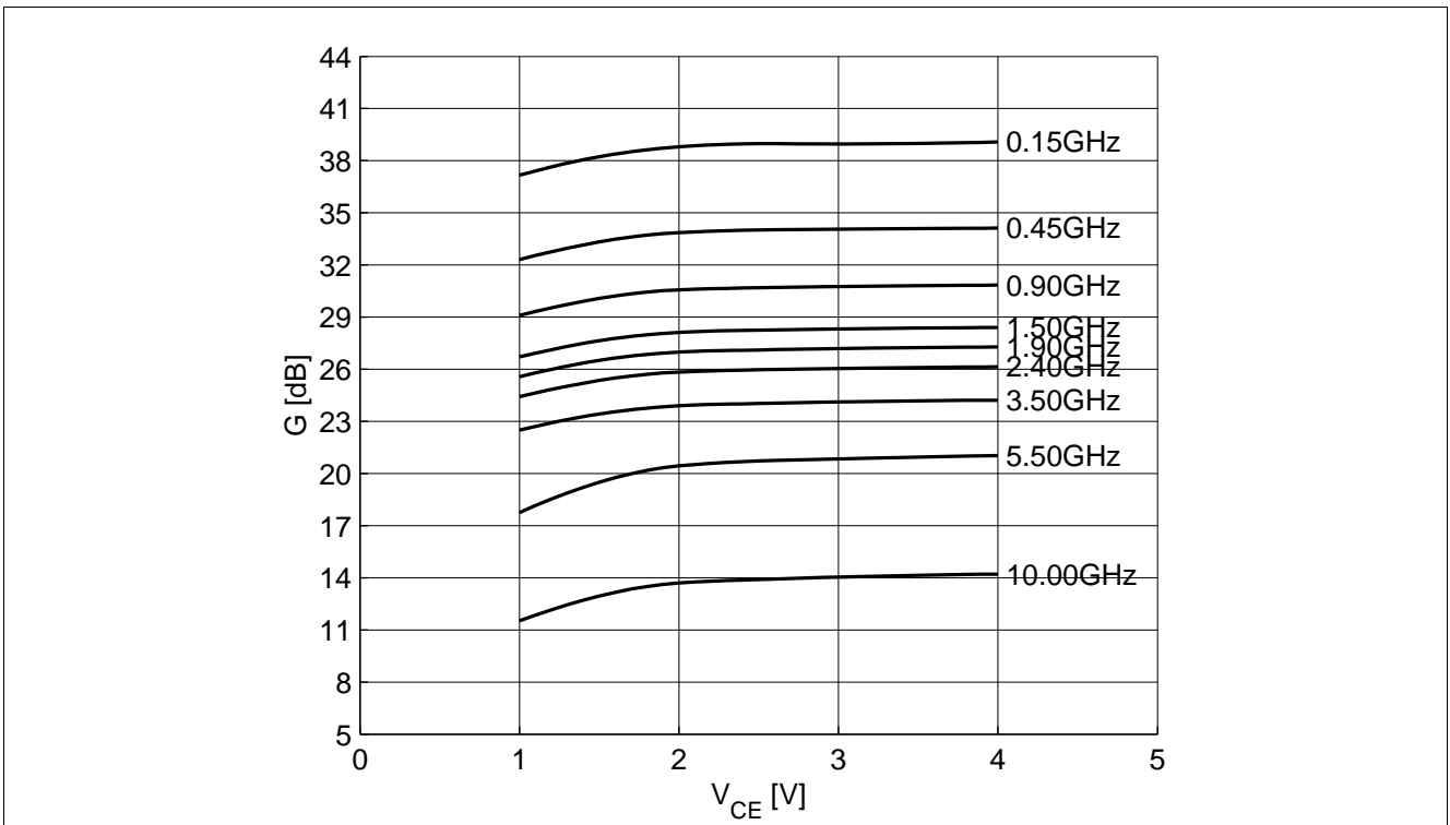
Figure 5-12 Maximum Power Gain G_{max} = f(V_{CE}) , I_C = 25 mA , f = Parameter in GHz
