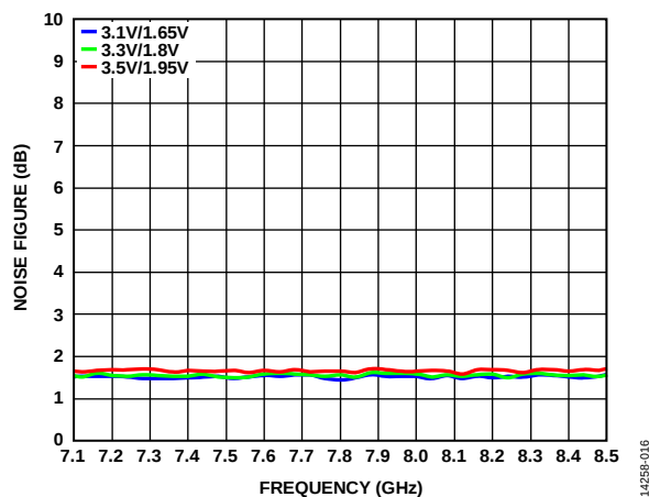
Figure 16. Noise Figure vs. Frequency for Various Supply Voltages
