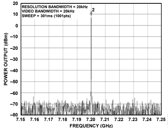
Figure 32. Results of the ADL5721 with an Input of 7.2 GHz at -15 dBm, BAND = 0 V
