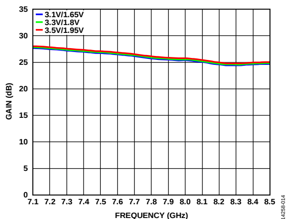
Figure 14. Gain vs. Frequency for Various Supply Voltages
