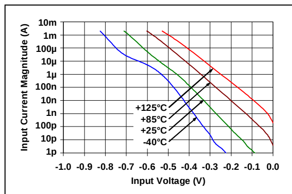
FIGURE 2-7: Input Current vs. Input Voltage.
