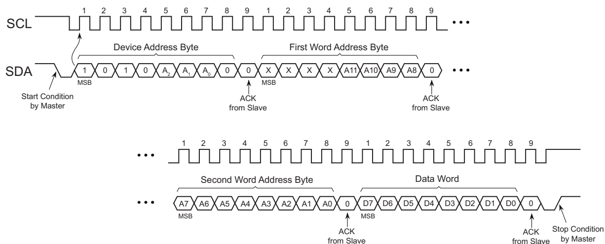
Figure 5-1. Byte Write
