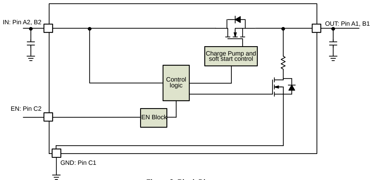
Figure 2. Block Diagram
