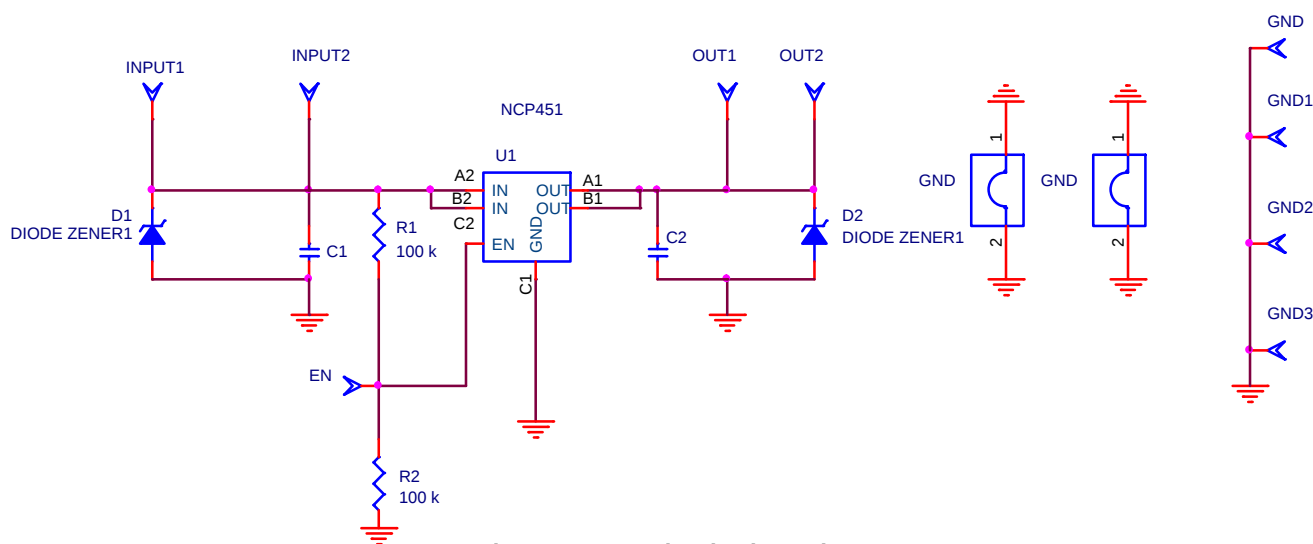
Figure 14. Demobard schematic
