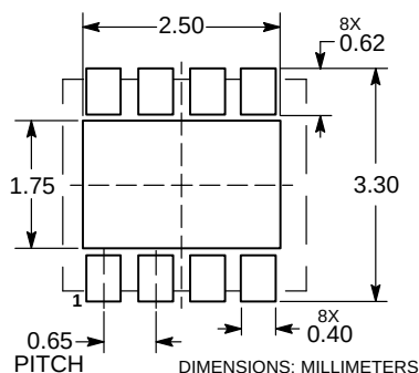
RECOMMENDED SOLDERING FOOTPRINT*
