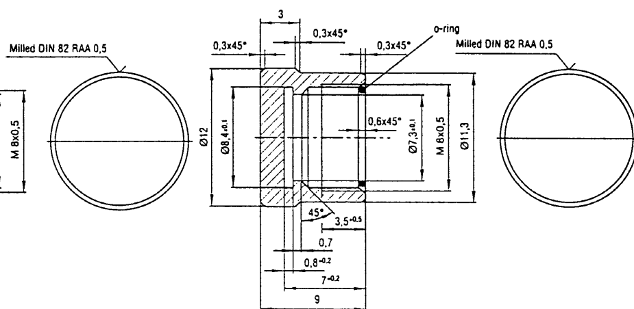
Dust cap: for pin connectors
