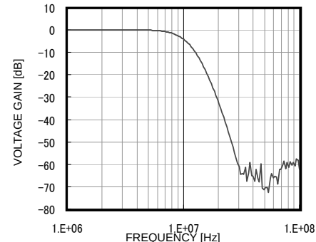
Fig. 24 Frequency Characteristic
