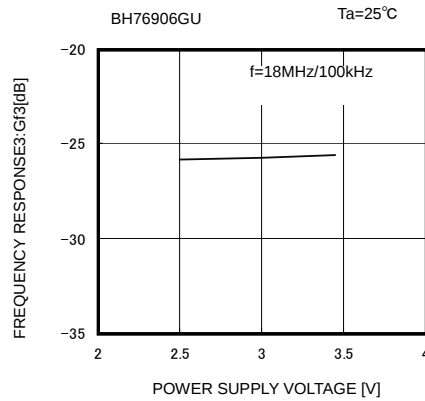
Fig. 32 Frequency Characteristic 3 vs Supply Voltage
