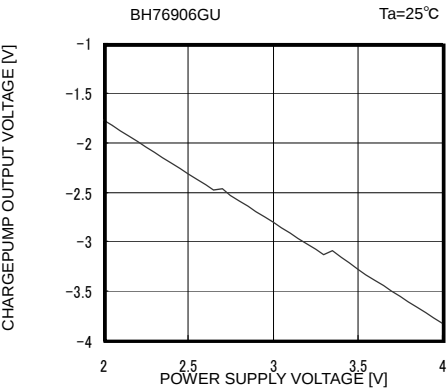
Fig. 41 Charge Pump Output Voltage vs Supply Voltage
