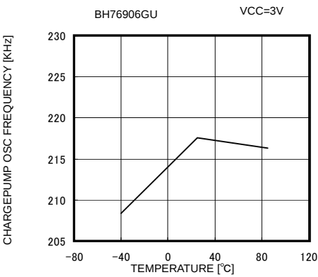
Fig. 40 Charge Pump Oscillation Frequency vs Ambient Temperature
