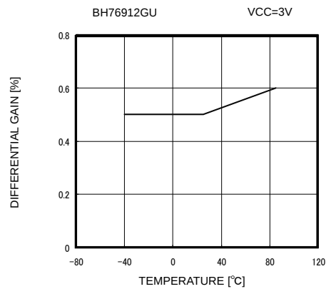
Fig. 46 Differential Gain vs Ambient Temperature
