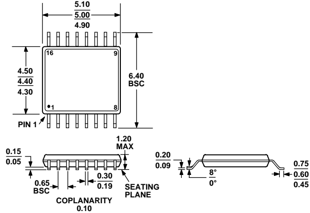
Figure 20. 16-Lead Thin Shrink Small Outline Package [TSSOP] (RU-16)
