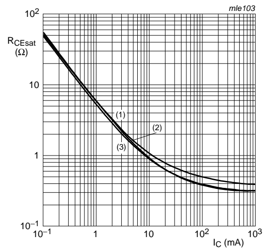
I_C/I_B = 20 (1) T_{amb} = 150\text{ }^\circ\text{C} (2) T_{amb} = 25\text{ }^\circ\text{C} (3) T_{amb} = -55\text{ }^\circ\text{C} Fig 9. Collector-emitter equivalent on-resistance as a function of collector current; typical values
