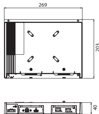
FPM-B700
