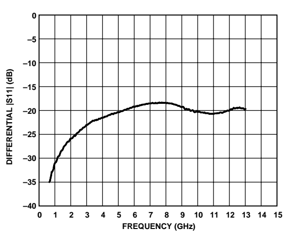
Figure 10. Differential |S 11 |
