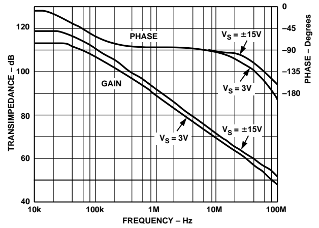
Figure 19. Open-Loop Transimpedance vs. Frequency (Relative to 1 \Omega )
