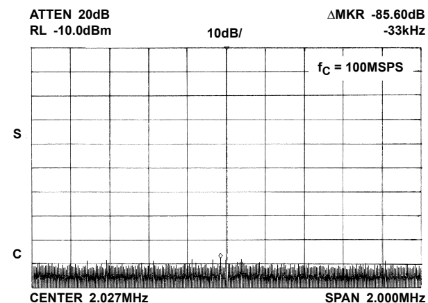
FIGURE 14. SPURIOUS FREE DYNAMIC RANGE = 85.60dBc
