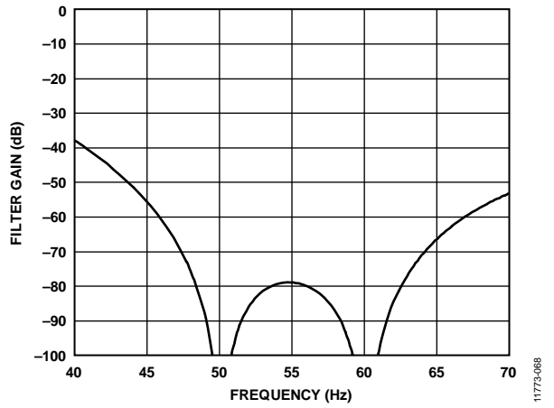
Figure 68. 16.667 SPS ODR, 60 ms Settling Time
