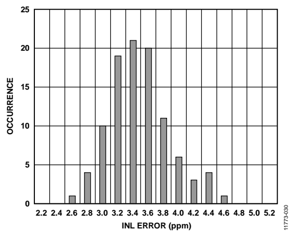
Figure 30. Integral Nonlinearity (INL) Distribution Histogram (Differential Input, V_{REF} = 5\text{ V} External)
