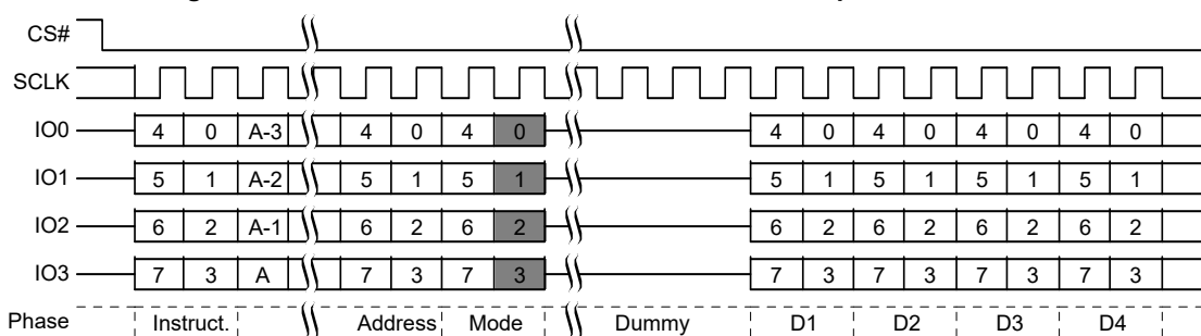
Figure 72. Quad I/O Read Initial Access Command Sequence QPI Mode
