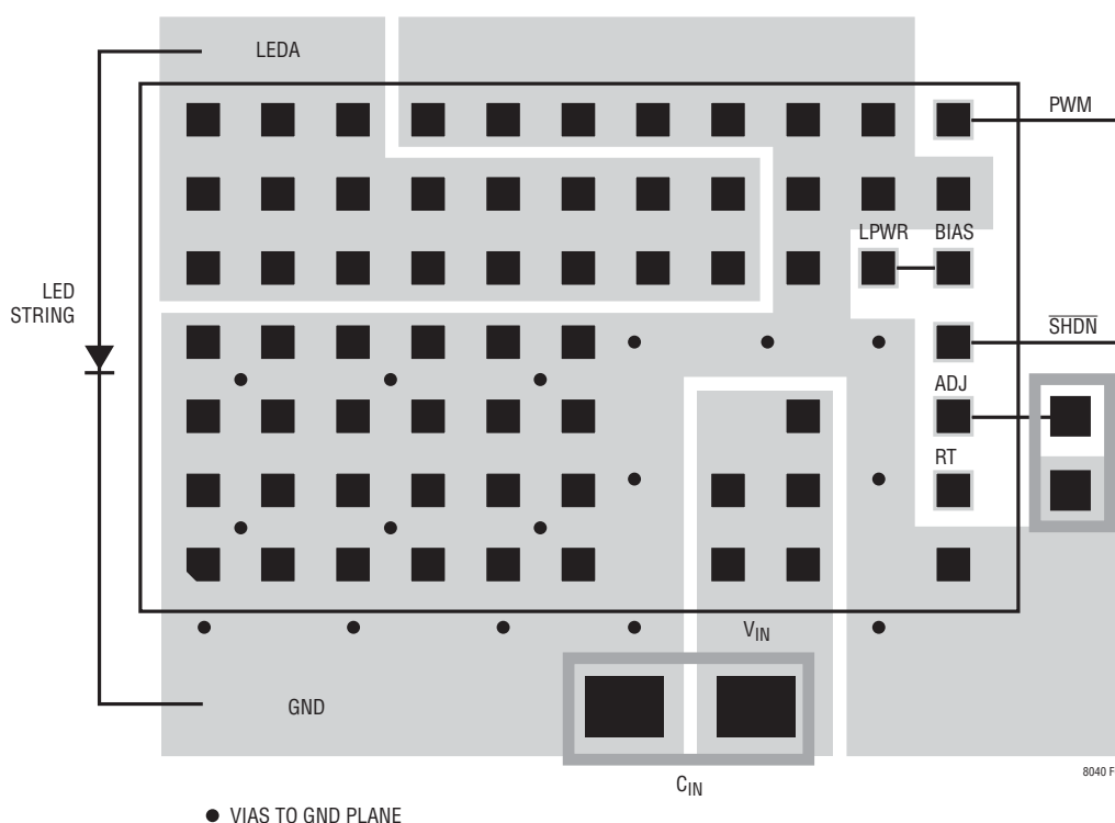
Figure 6. Suggested Layout
