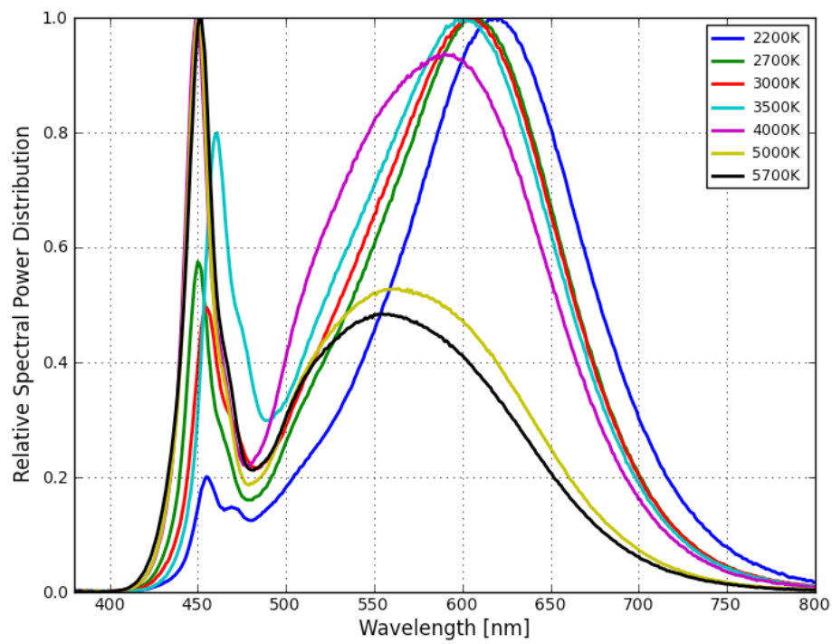
Figure 1: Typical relative intensity vs. wavelength for LUXEON 3535L color spectrum 80CRI at 100mA, T j =25°C.
