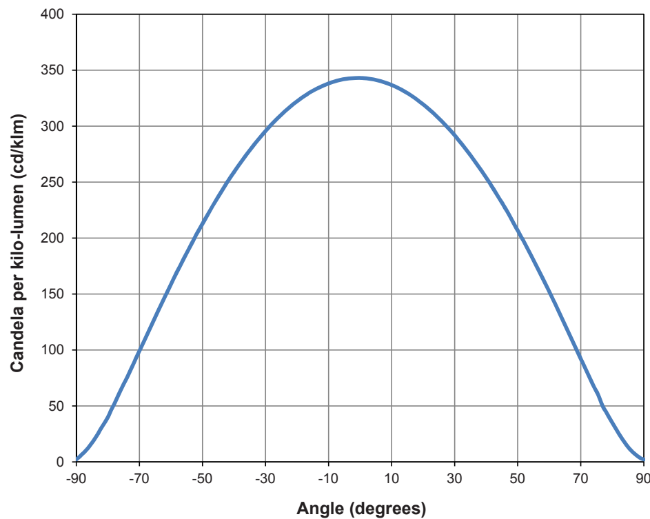
Figure 2: Typical radiation pattern for LUXEON XF-3535L at 100mA/LED, T j =25°C.
