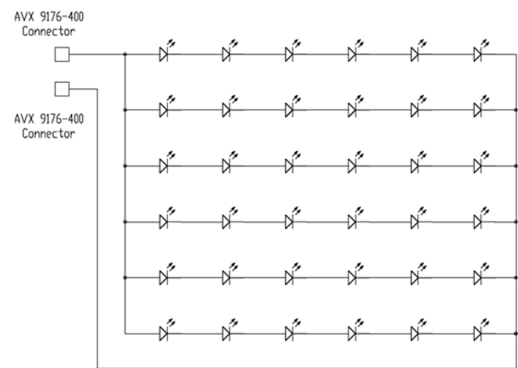
Figure 7: Electrical circuit diagram for L235-xyyAHLGBBAC0.
