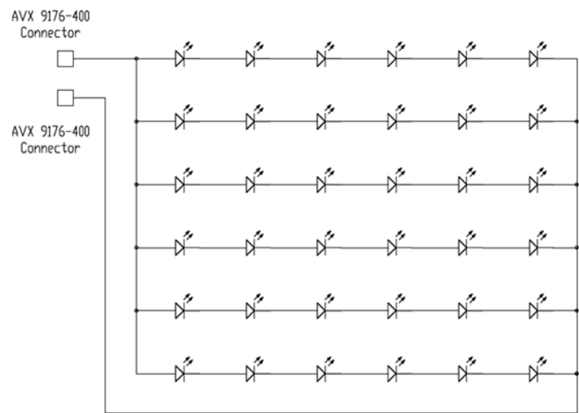
Figure 11: Electrical circuit diagram for L235-xyyyAHLCBAC0.
