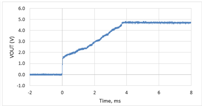
Figure 4.23. 5 V–5 V VOUT Startup vs.Time (No Load)
