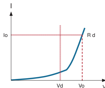
Figure - LED I-V Curve
