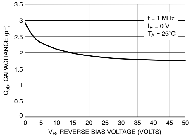
Figure 103. Output Capacitance
