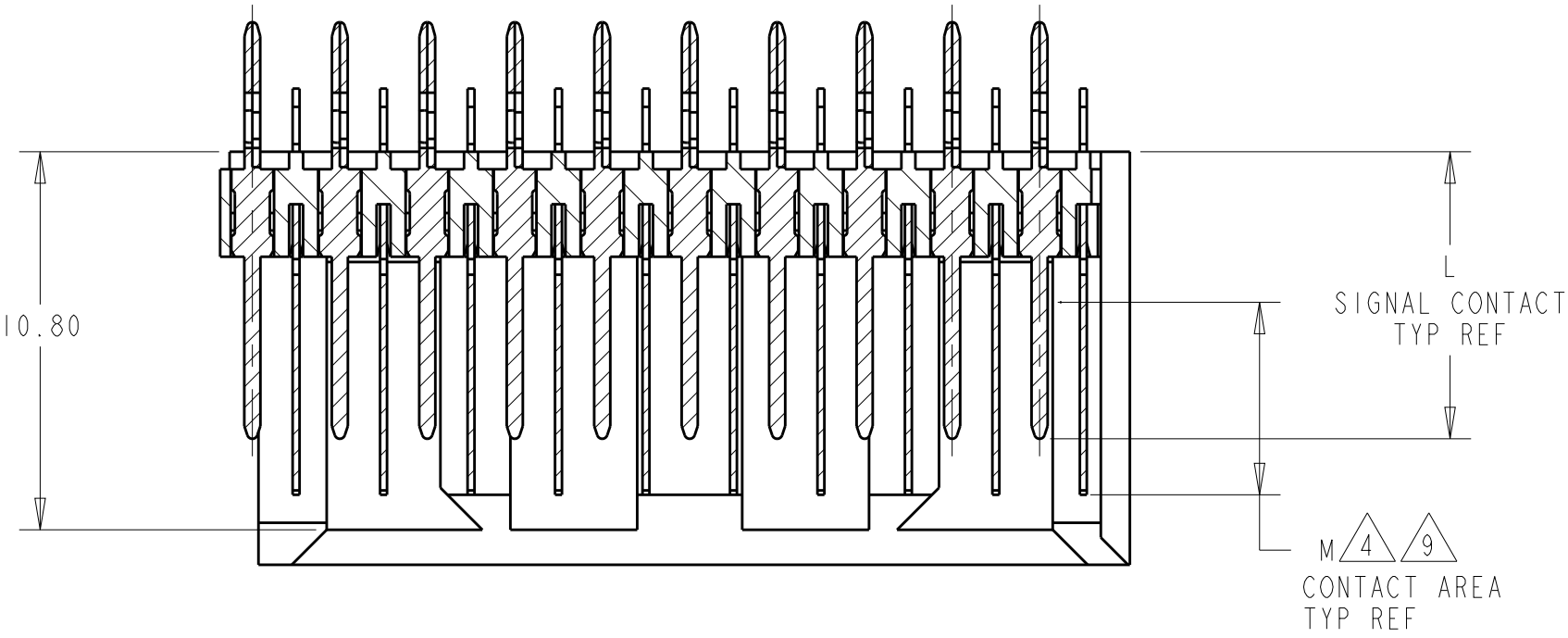
SECTION B-B
