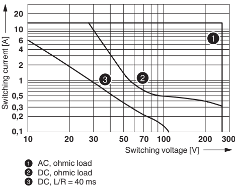
Interrupting rating
