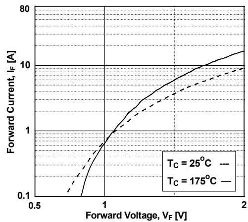
Figure 18. Forward Characteristics
