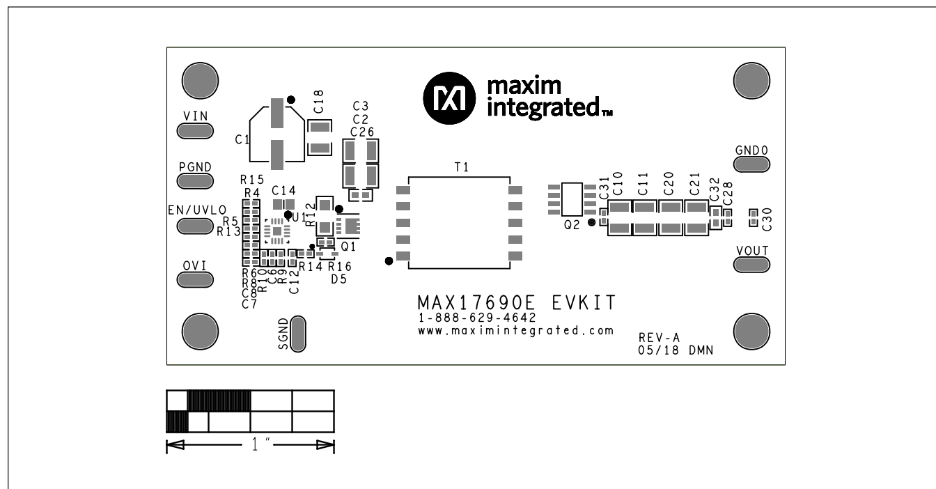
Silk_Top
