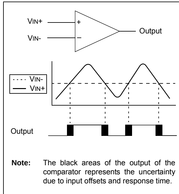
FIGURE 17-1: SINGLE COMPARATOR
