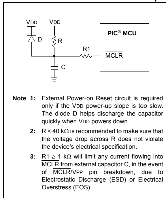
FIGURE 22-2: EXTERNAL POWER-ON RESET CIRCUIT (FOR SLOW V_{DD} POWER-UP)
