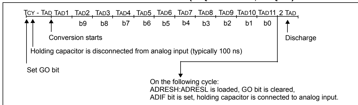
FIGURE 16-3: A/D CONVERSION TAD CYCLES (ACQT<2:0> = 000, TACQ = 0)
