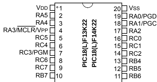
FIGURE 1: 20-PIN PDIP, SSOP, SOIC
