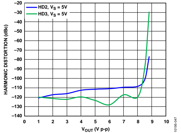
Figure 40. Harmonic Distortion vs. V_{OUT,dm} , f = 10 kHz
