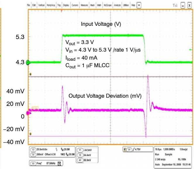
Figure 26. Line Transient Response 3.3 V/40 mA
