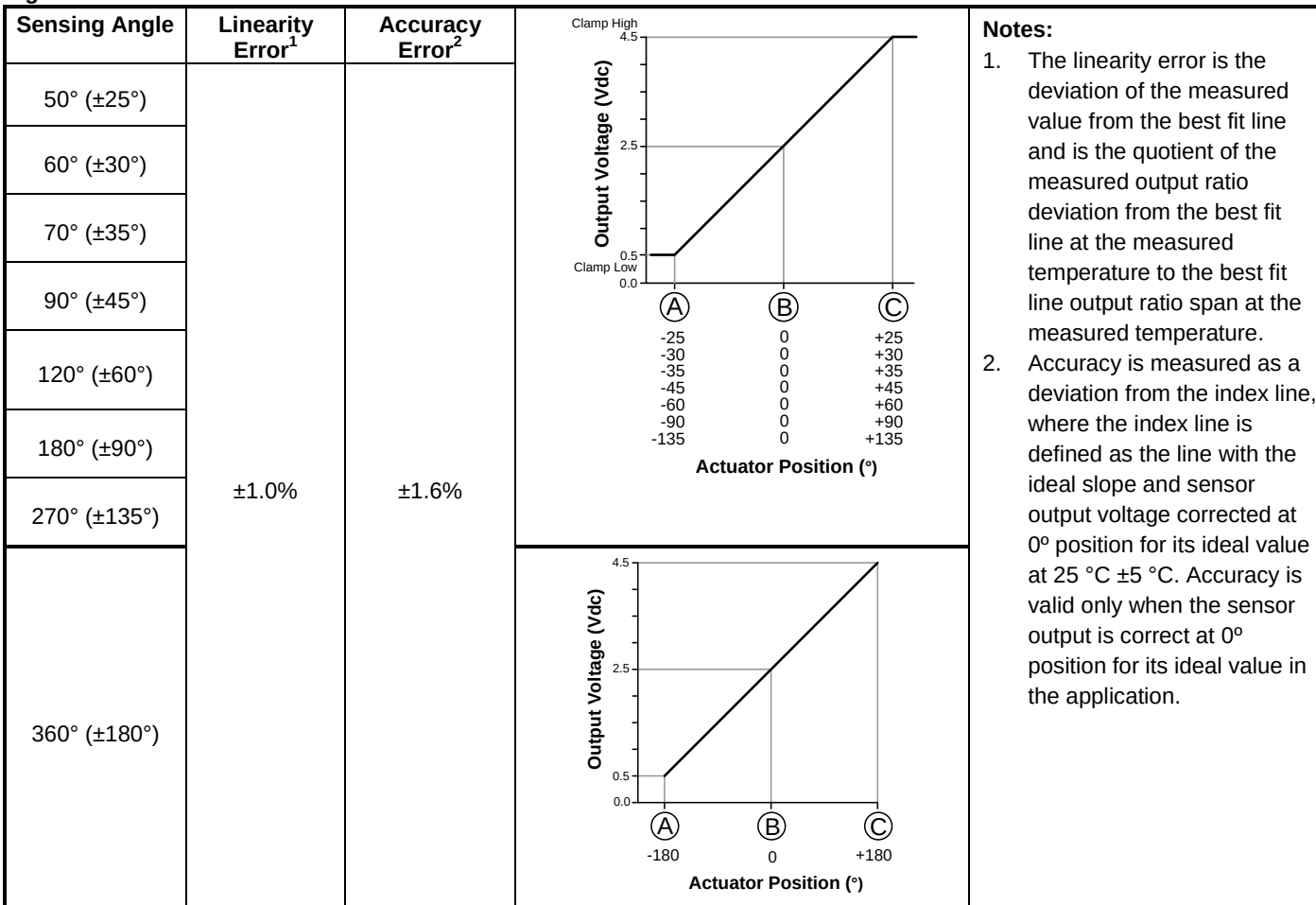
Figure 2. Functional Characteristics
