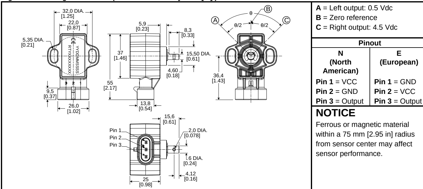
Figure 1. Mounting Dimensions (For Reference Only: mm/[in].)
