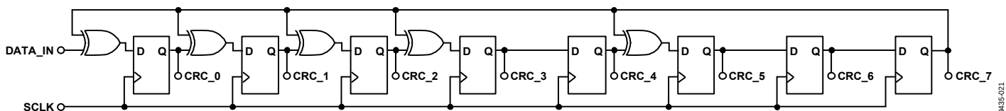
Figure 40. CRC Implementation
