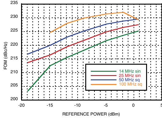
Figure 15. Integer-N Performance at 704 MHz [5]
