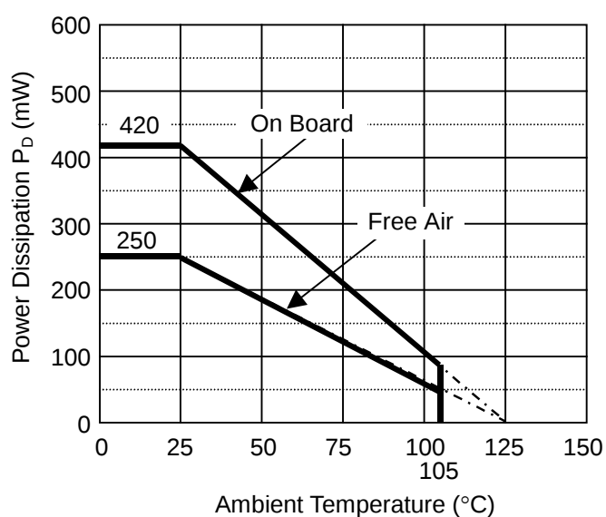
Power Dissipation
