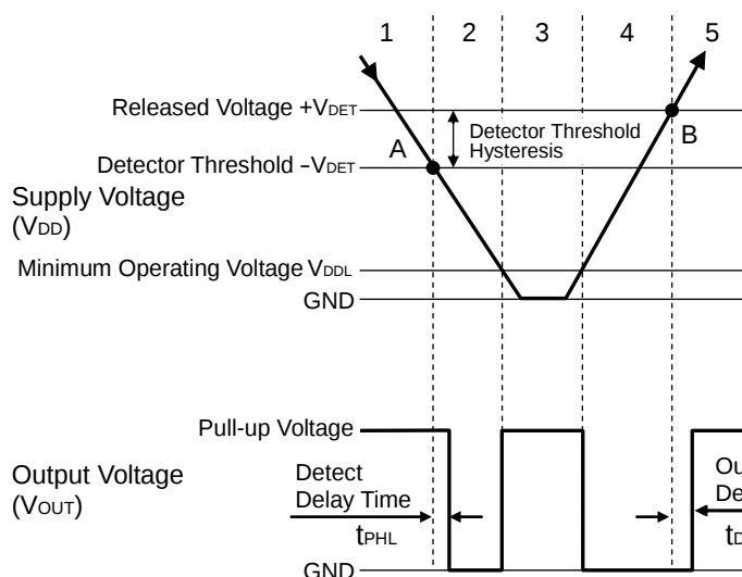
Operation Diagram
