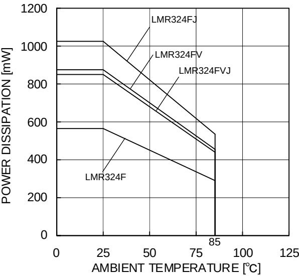
Figure 50. Derating curve
