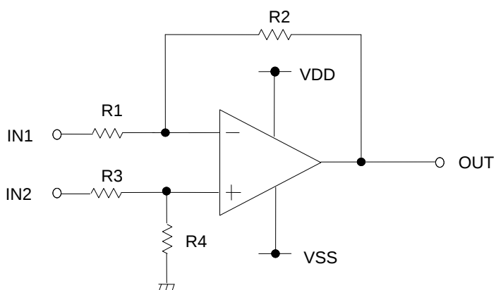
Figure 82. Differential amplifier
