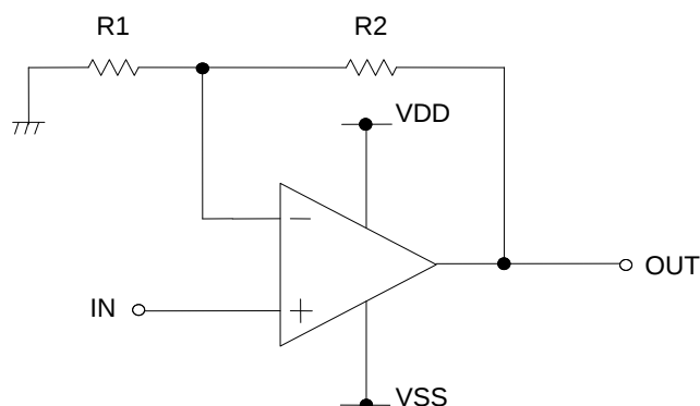
Figure 80. Non-inverting amplifier
