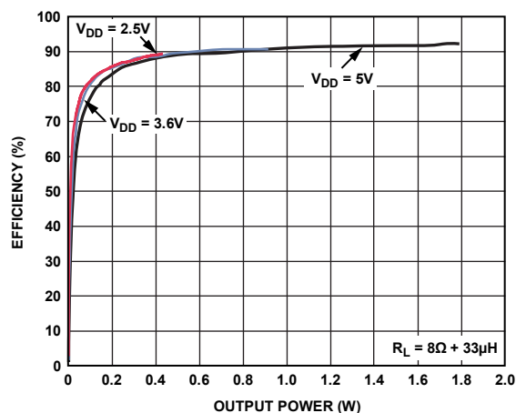
Figure 19. Efficiency vs. Output Power into R_L = 8\Omega + 33\mu\text{H}
