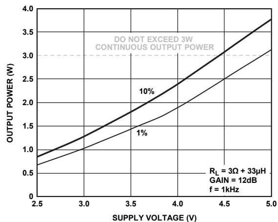
Figure 16. Maximum Output Power vs. Supply Voltage, R_L = 3\Omega + 33\mu\text{H} , Gain = 12 dB
