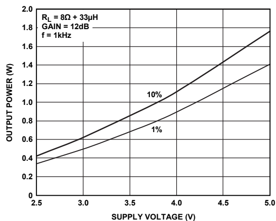
Figure 18. Maximum Output Power vs. Supply Voltage, R_L = 8\Omega + 33\mu\text{H} , Gain = 12 dB
