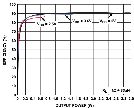
Figure 20. Efficiency vs. Output Power into R_L = 4\Omega + 33\mu\text{H}
