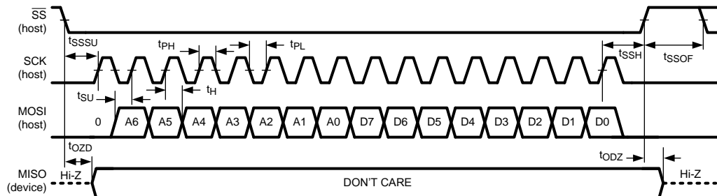
Figure 4. SPI Write
