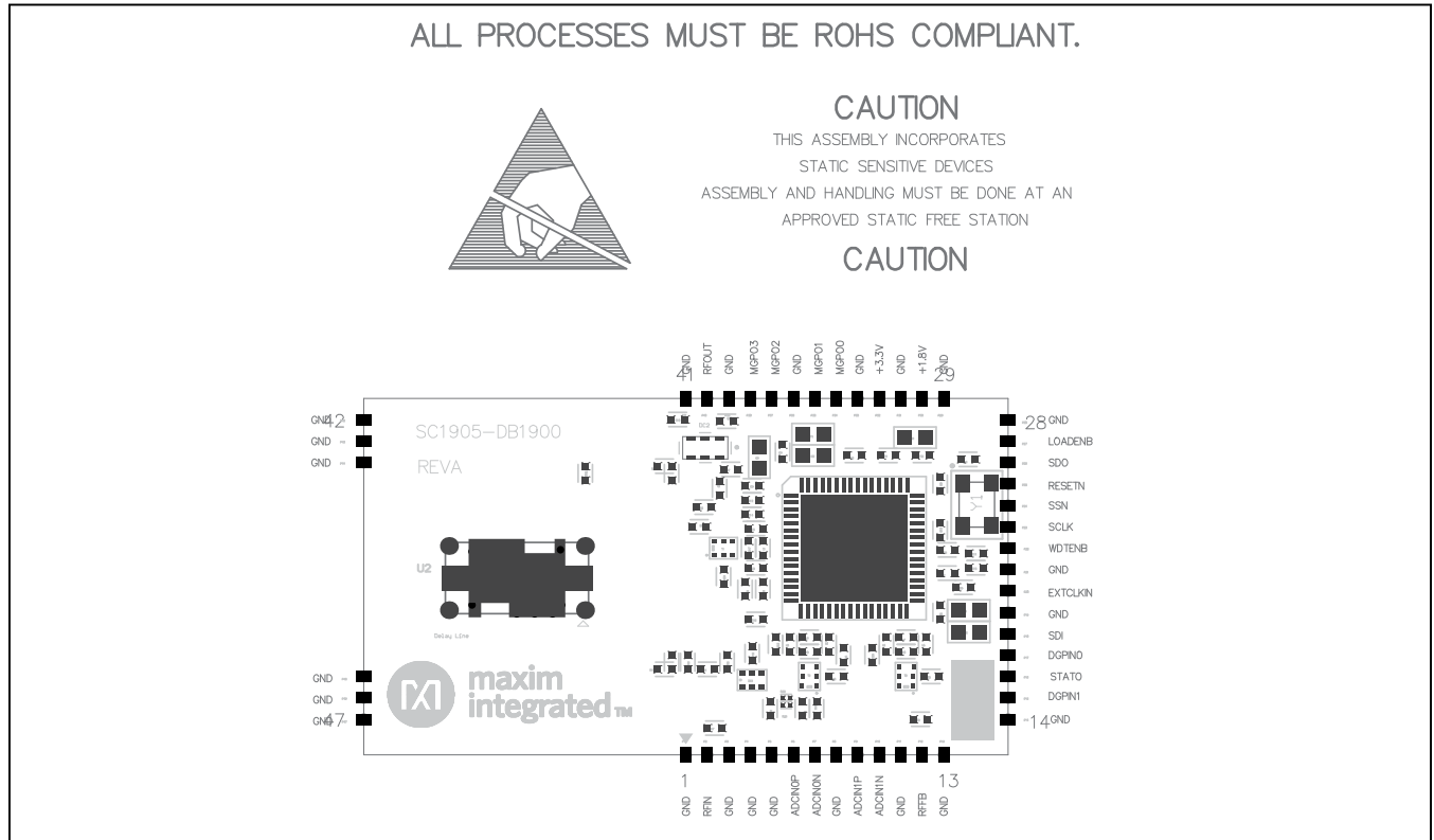
SC1905-DB1900—Assembly Drawing
